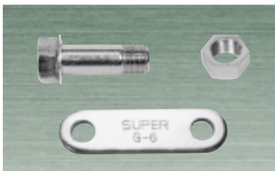
Bolt and nut (One set for 6 pieces)
