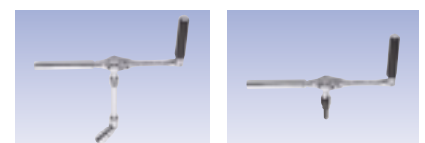
Combination with extension bar, universal joint and socket.
